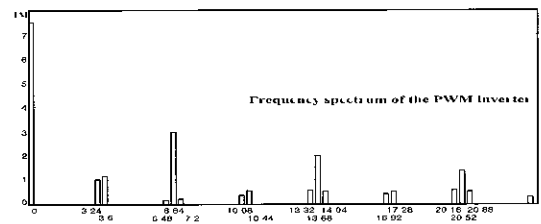
(b) PWM 인버터 입력 측 직류링크 전류(60Hz) (b) Dc link current of PWM inverter input side at 60Hz of fundamental frequency
